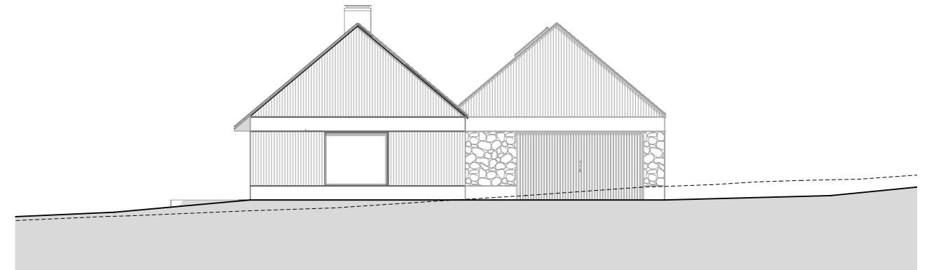
EASTERN ELEVATION
