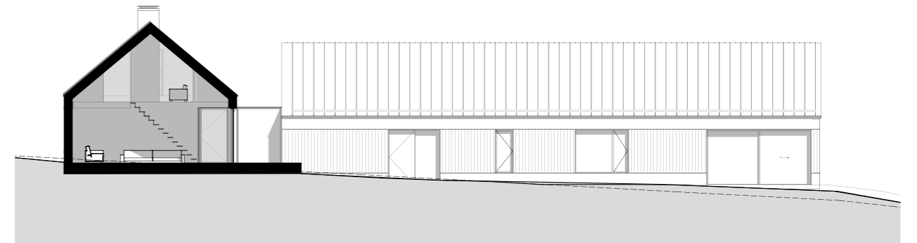
WESTERN SECTIONAL ELEVATION
