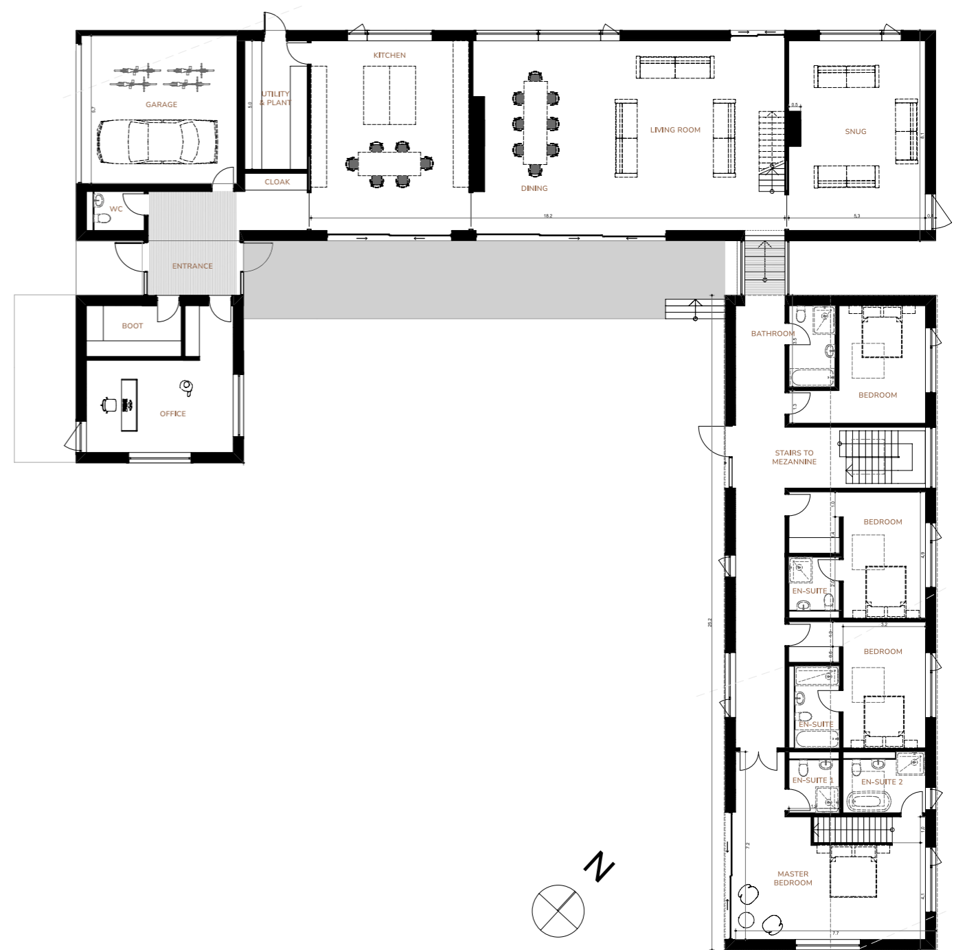
1_GROUND FLOOR
