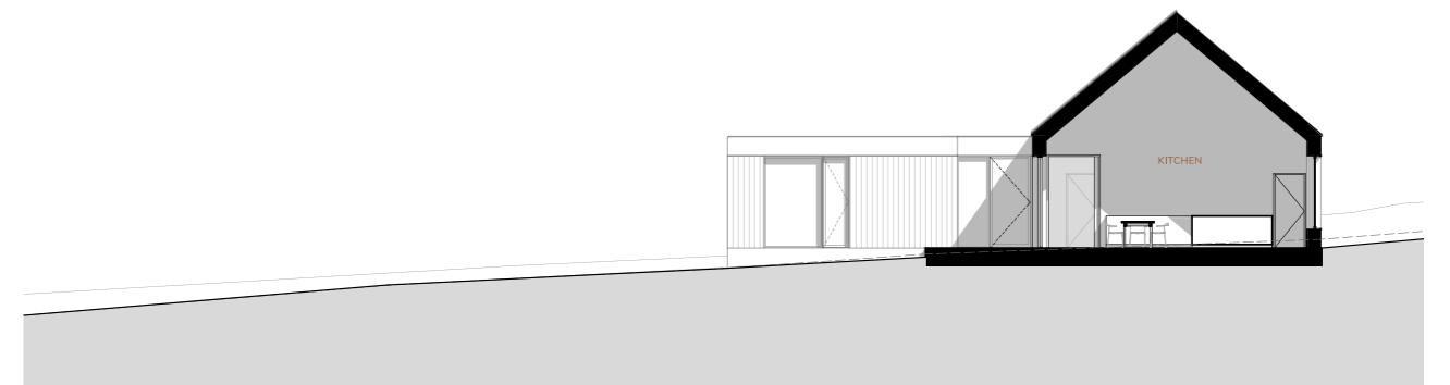
EASTERN SECTIONAL ELEVATION
