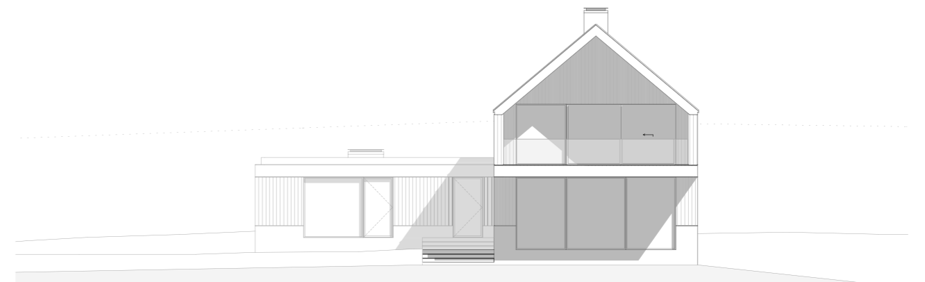
SOUTH ELEVATION
