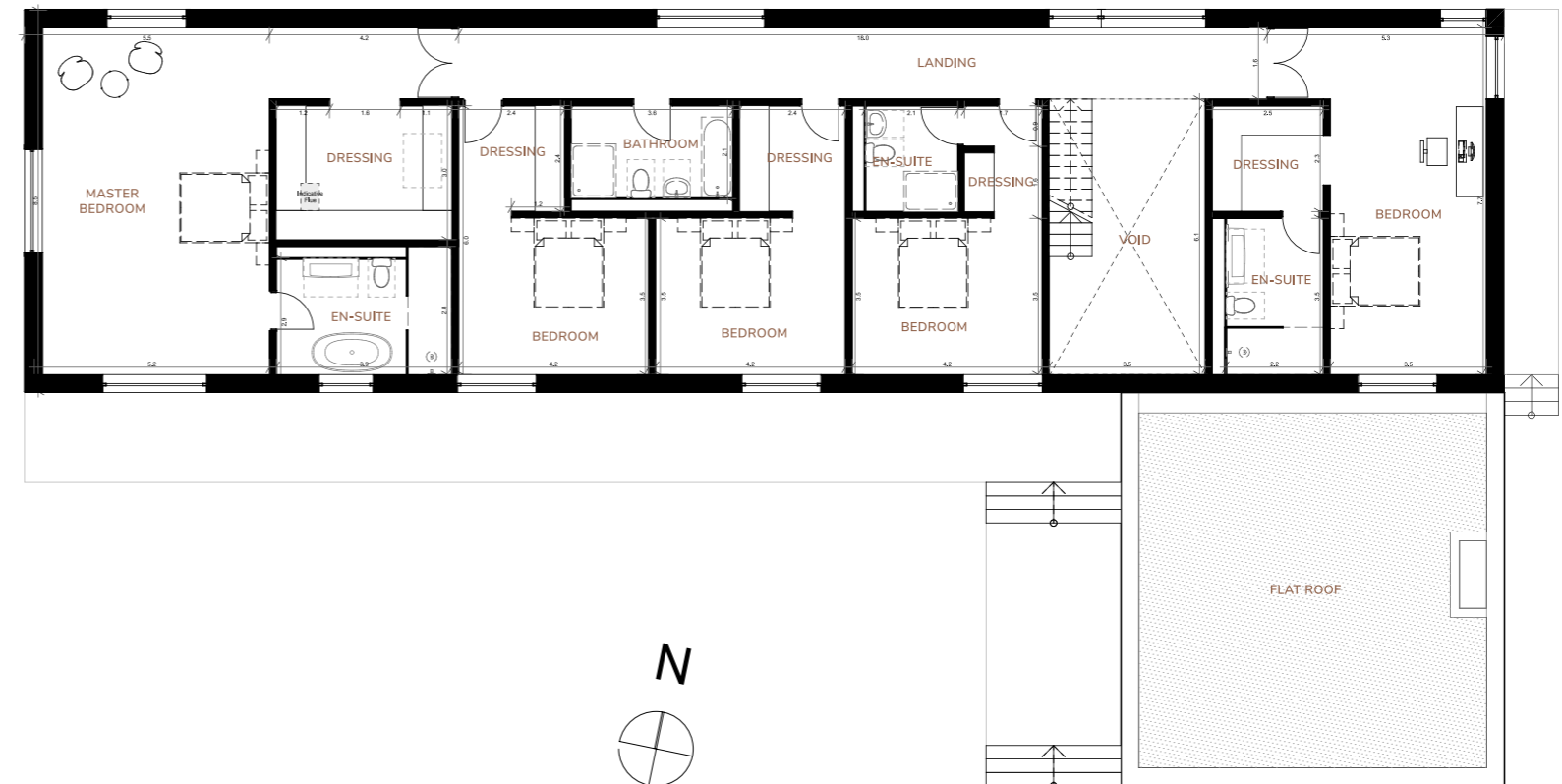
2_FIRST FLOOR PLAN
